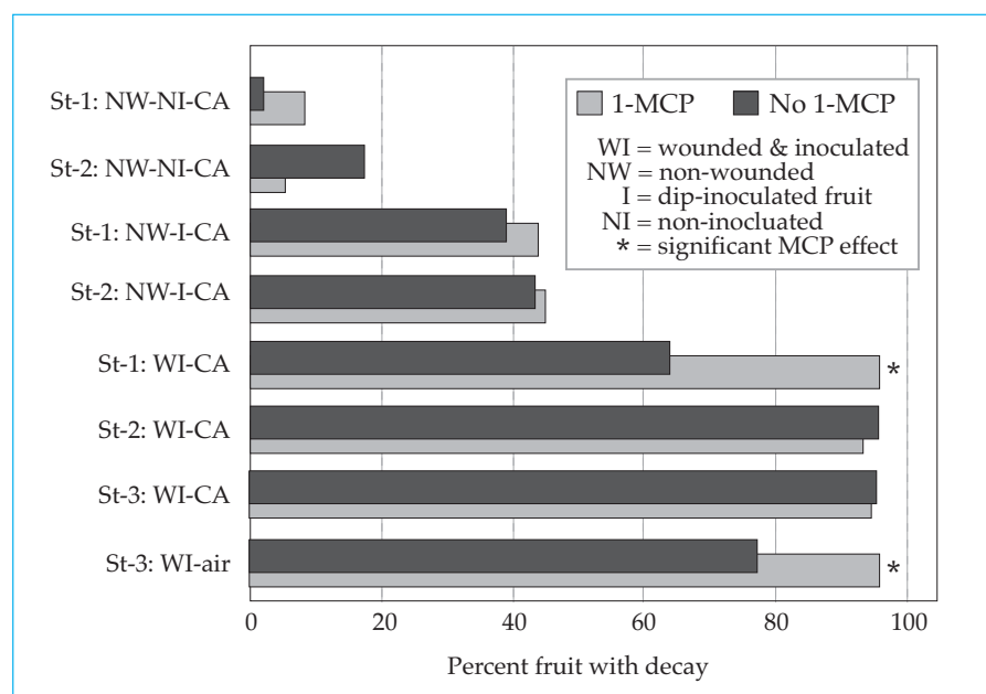
Figure 1. Effects of 1-MCP treatment on incidence of decay in experiments initiated in fall of 2003. Treated and non-treated fruit were held in three different CA storages, and a comparable sample was held in air storage at St-3. None of the fruit in these experiments received any postharvest fungicide treatment.
