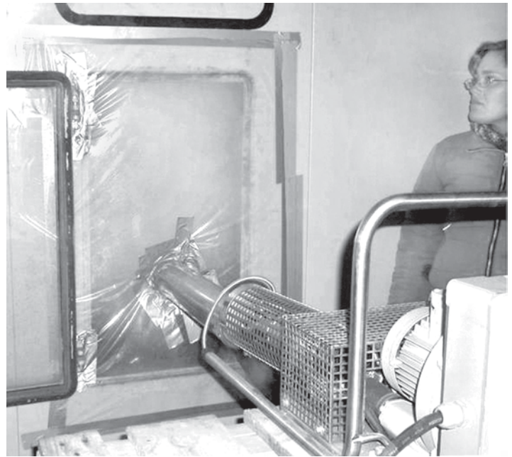
Figure 1. Thermofogging of a CA storage room with DPA. Photo provided by Pace International, LLC. Artwork, photographs and designs may not be copied, reproduced or used in any way without written authorization from Pace International, LLC. © 2007 Pace International LLC - All Rights Reserved
